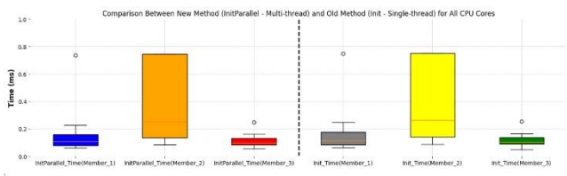
Figure 8: Performance Comparison of both the new multi-threaded method (InitParallel) and the old single-threaded method (Init) across 16 CPU Cores.
